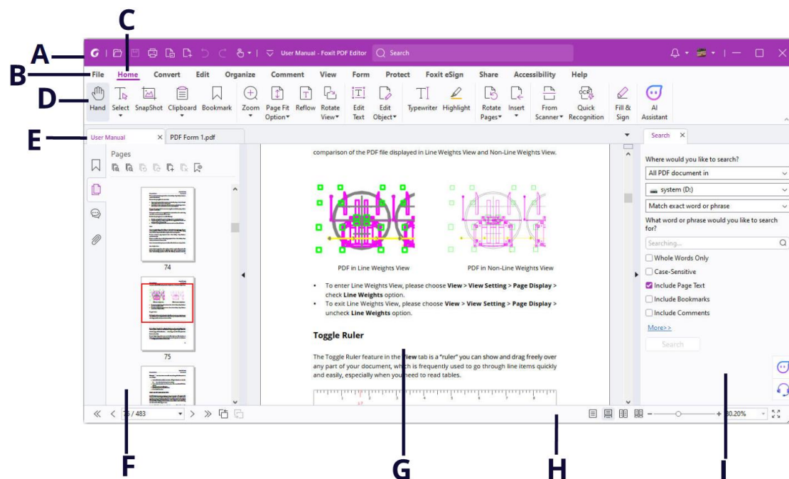
User Interface
