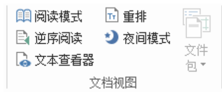
视图菜单
