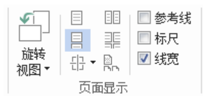
视图菜单
