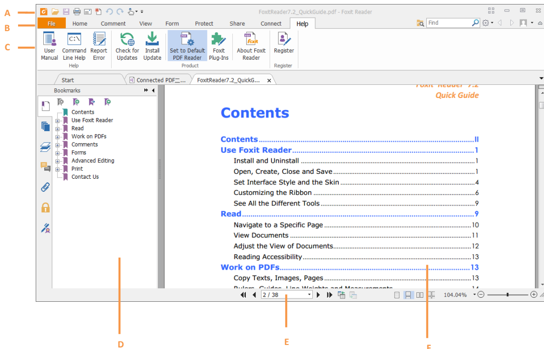
Fig. 1 User Interface
