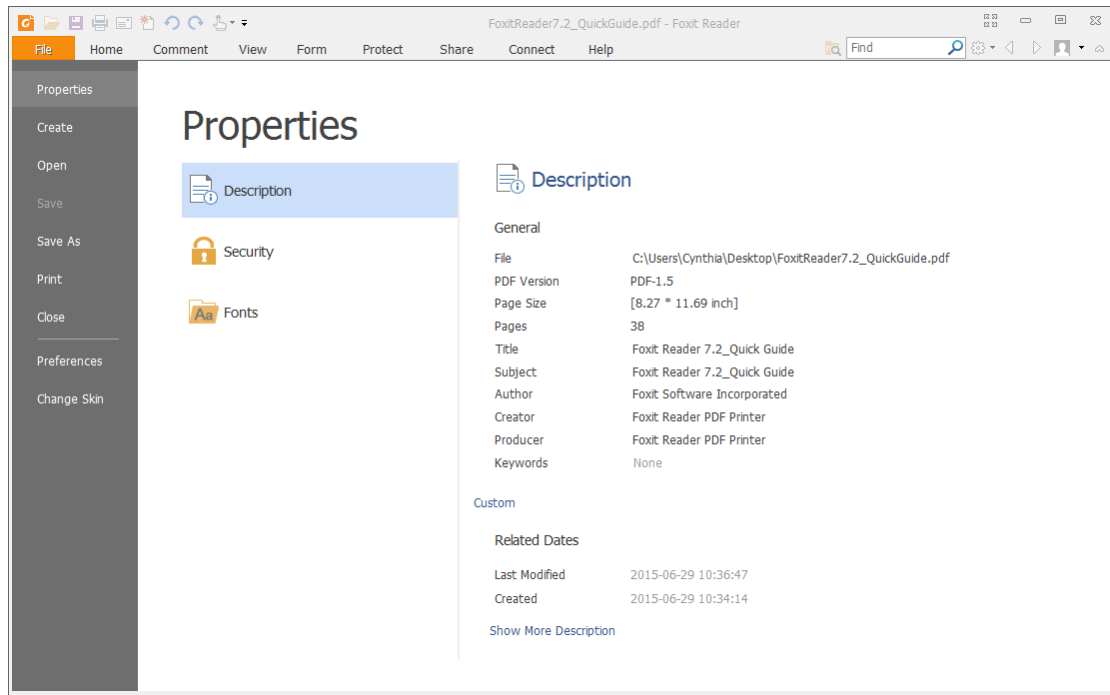
Fig. 2 File Page
