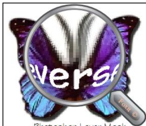
Fisheye Magnifier
